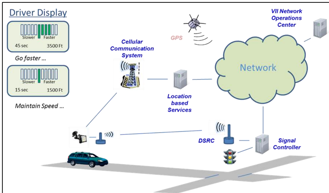
Figure 1 - Multipath SPAT Broadcast System Architecture
